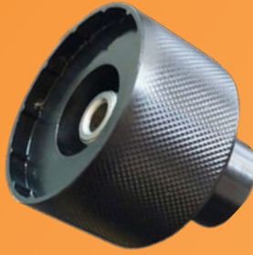
RC-BF52 Product Name: E-Bike Hub & Chaining Removal Tool for ISIS 47T Motor Systems
